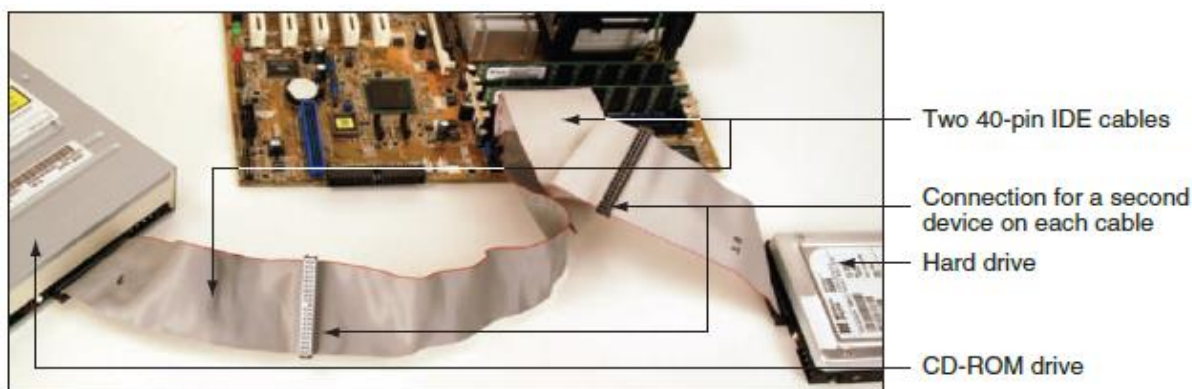
Figure (18) Two PATA devices connected to a motherboard using both PATA or IDE connections and two cables
