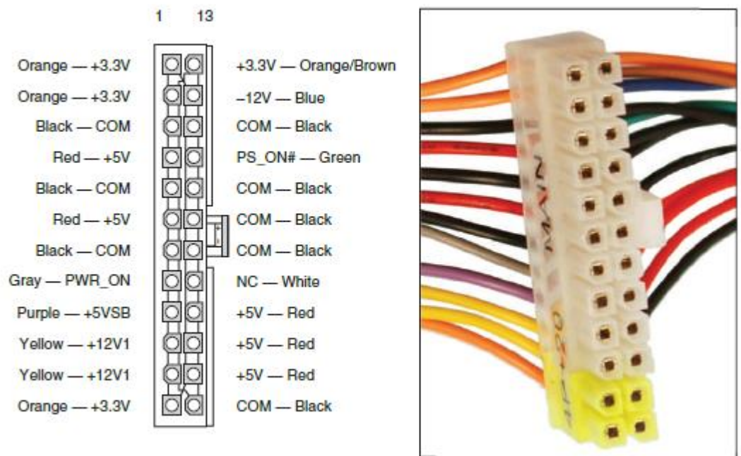
Figure (15) P1 24-pin power connector follows ATX Version 2.2 and higher standards
